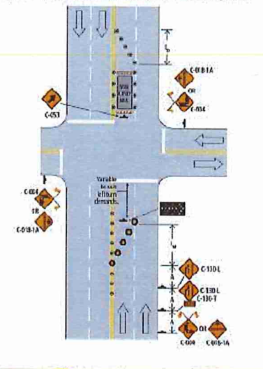
Figure 11.7: Left Lane Closure Per Side – Multiple Intersections – Short and Long Durations
