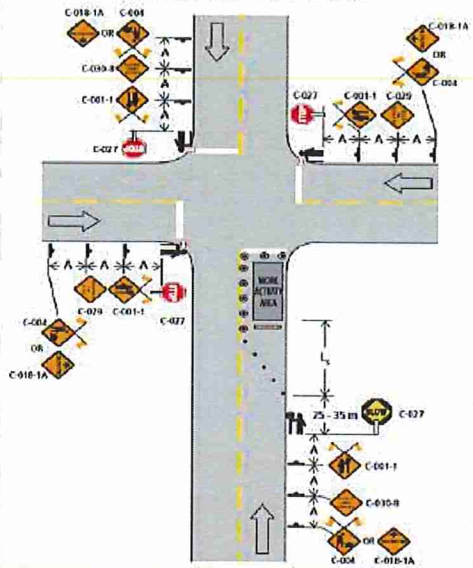
Figure 11.2: Intersection Lane Closure – Two-Lane, Two-Way Roadway with TCPs (Near Side) – Short and Long Duration
