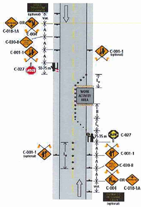
Figure 7.8: Lane Closure with TCPs – Single Lane Alternating – Short and Long Durations
